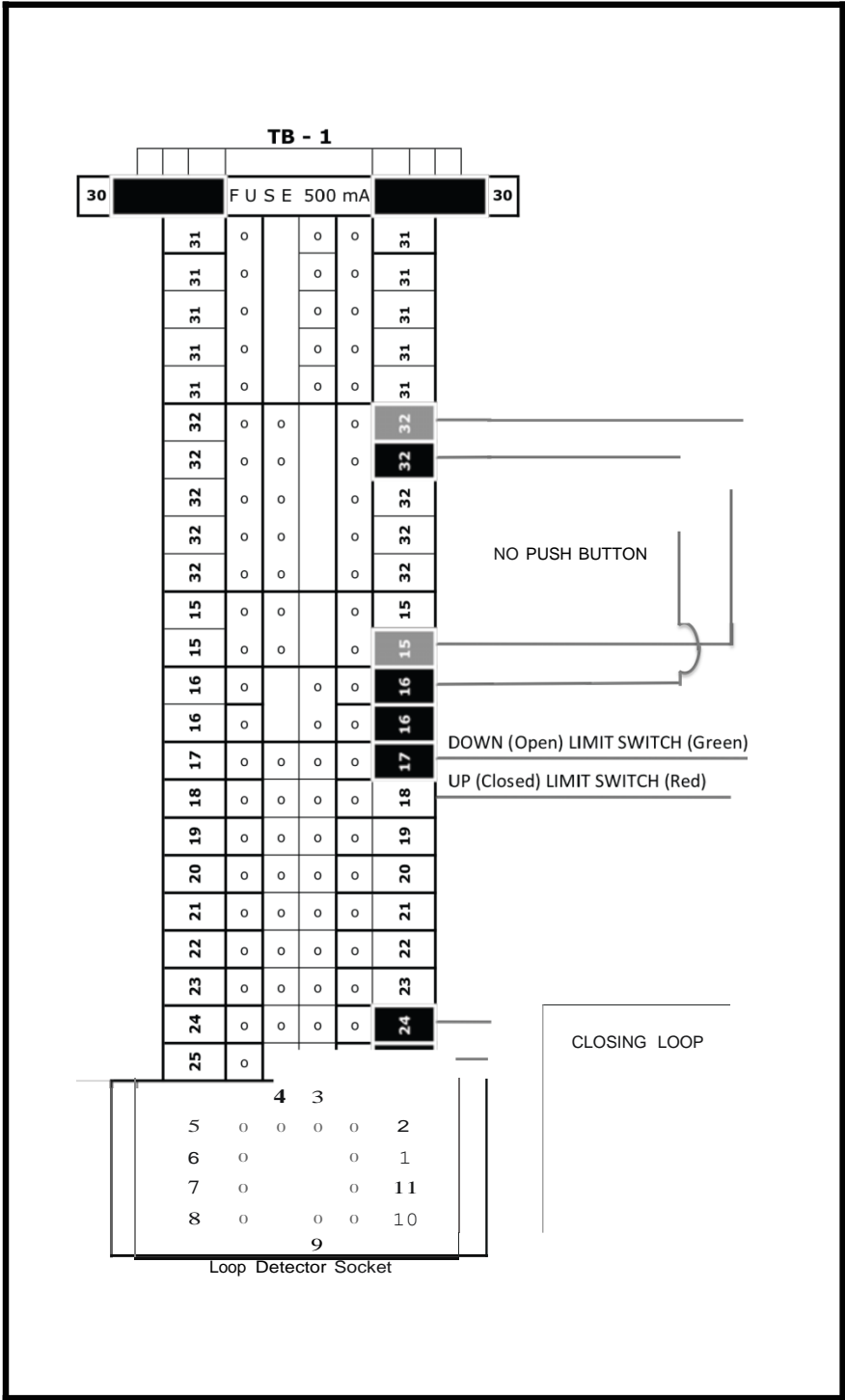
Figure 34 TB 1 Terminal Block, Installation Wiring, Control Cabinet
