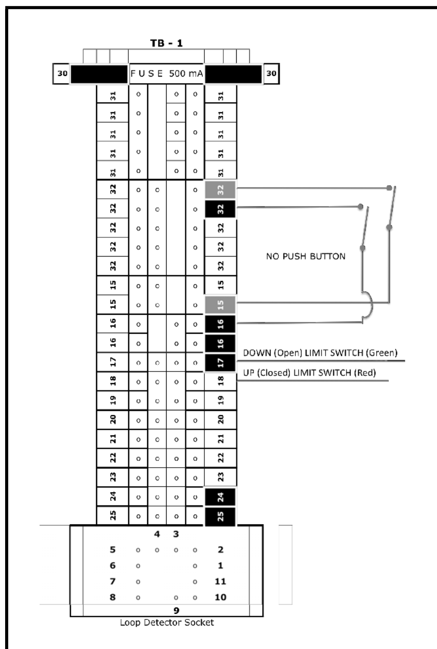
Figure 30 Limit Switch Wiring (Usually Performed at Factory)
