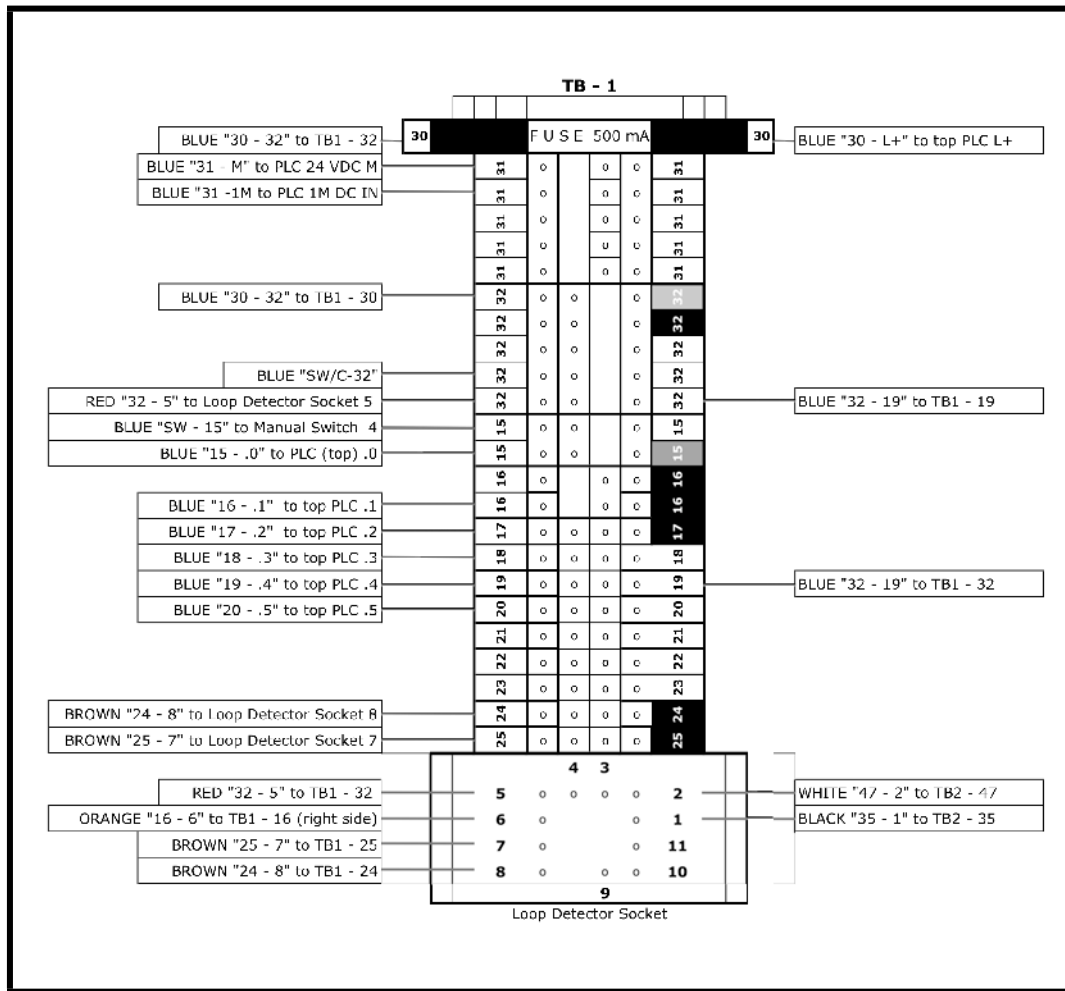
Figure 35 TB 1 Terminal Block, Factory Wiring, Control Cabinet
