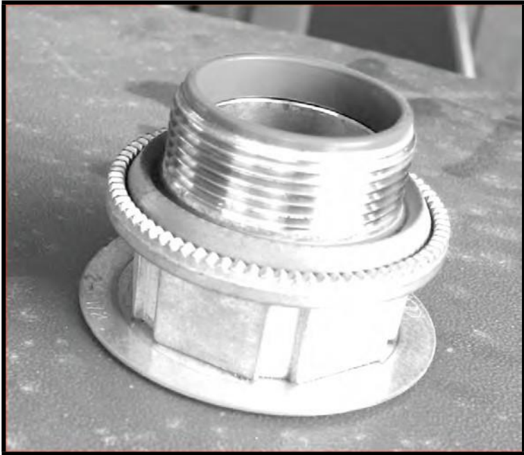
Figure 27 Assembled Traffic Control Mounting Adapter, Control Cabinet
