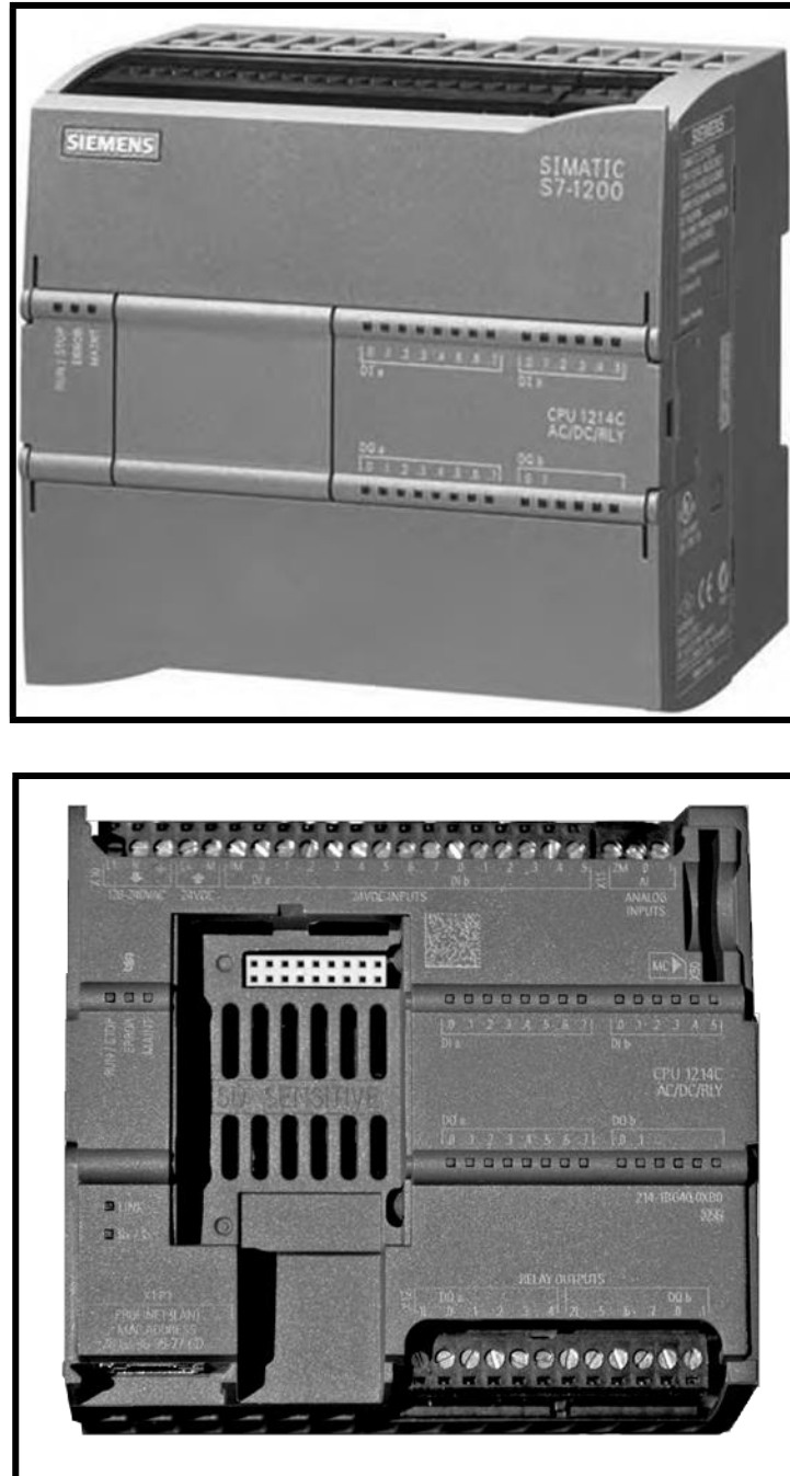
Figure 32 Siemens S7-1200 PLC, Control Cabinet -- With (Top) and Without (Bottom) Covers Removed
