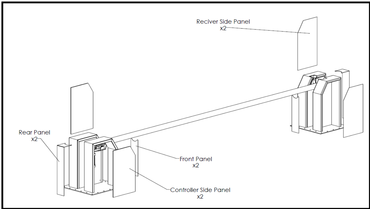
Figure 2 DBA Product Family Major Component Identification
